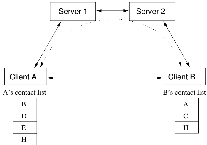
Figure 1.1: IM communications models
